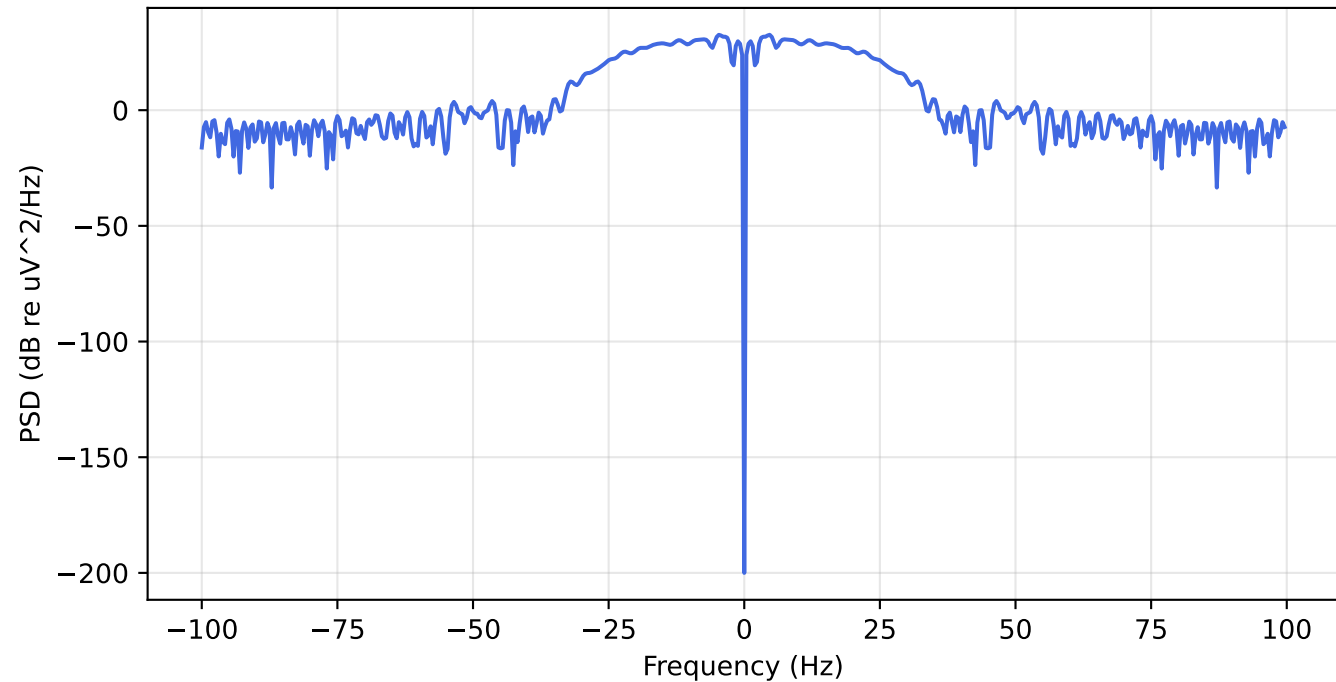
PSD of the average PQRST complex ( S_d )
